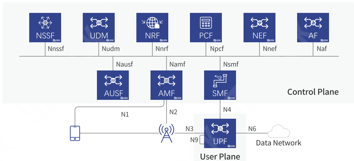
5GC Architecture
