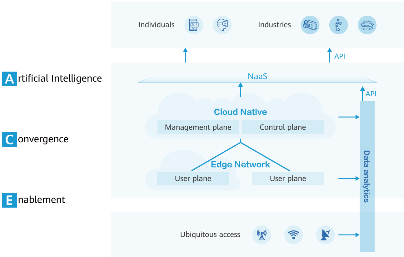
Figure 2-1: 5G-Advanced network architecture
